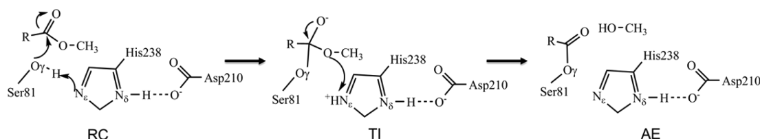
Figure 1. Acylation reaction mechanism in SABP2 with the catalytic triad involving Ser-81, His-238, and Asp-210. RC represents the reactant complex, TI the tetrahedral intermediate, and AE the acyl-enzyme complex. SABP2 can catalyze reactions for a number of substrates, including methyl salicylate (MeSA), 21,25 methyl jasmonate (MeJA), 21,25 methyl indole-3-acetic acid ester (MeIAA), 21,25 acibenzolar-S-methyl, 28 4-methylumbelliferone butyrate, 23 p -nitrophenyl (pNP) palmitate, pNP myristate, pNP butyrate, 23 and pNP acetate. 27 Here we demonstrate that methyl benzoate (MeBA) is also a substrate of SABP2, and the increase in catalytic efficiency upon going from MeBA to MeSA is likely due to the participation of substrate-assisted catalysis.
