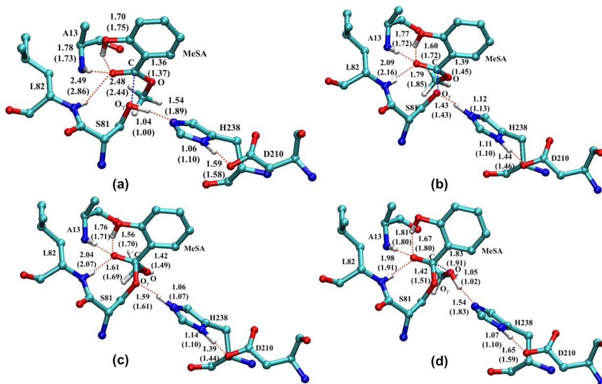
Figure 3. Results from the benchmark calculations for SABP2 complexed with MeSA. Numbers within parentheses are obtained from the SCC-DFTB/MM geometry optimization with dispersion correction; those without parentheses are obtained from the B3LYP/6-31G(d,p)/MM geometry optimization. Most hydrogen atoms have been omitted for the sake of clarity. (a) Reactant state obtained via adiabatic mapping. (b) Structure near transition state 1 obtained via adiabatic mapping. (c) Tetrahedral intermediate obtained via adiabatic mapping. (d) Structure near transition state 2. All distances are in angstroms.
