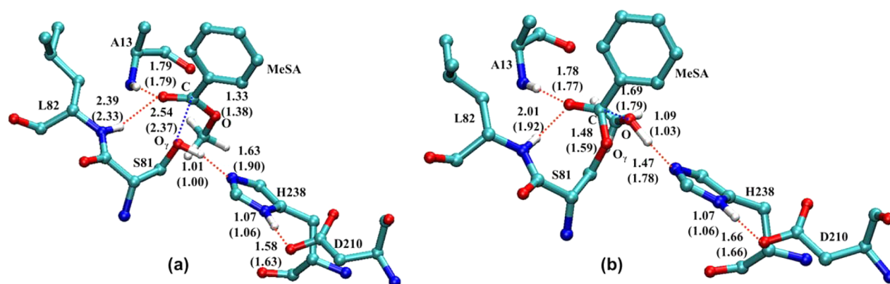
Figure 5. Results from the benchmark calculations for SABP2 complexed with MeBA. Numbers within parentheses are obtained from the SCC-DFTB/MM geometry optimization with dispersion correction; those without parentheses are obtained from the B3LYP/6-31G(d,p)/MM geometry optimization. (a) Reactant state obtained via adiabatic mapping. (b) Structure near the transition state (TS). All distances are in angstroms.
