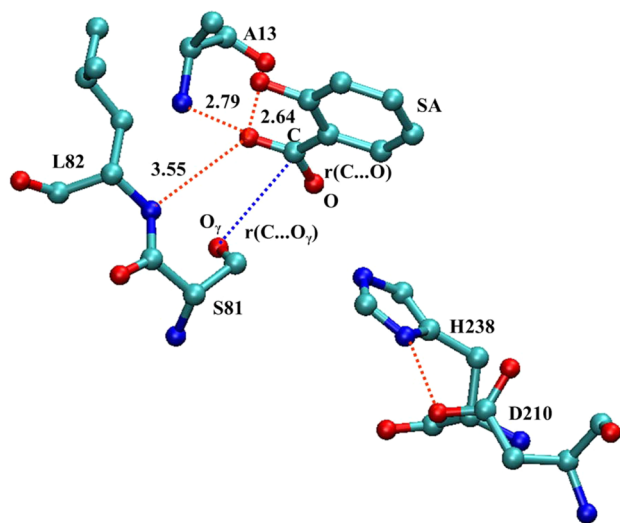
Figure 2. Active site of SABP2 from the X-ray crystal structure (Protein Data Bank entry 1Y7I) obtained in ref 21. The Reaction coordinate is RC = r(C \cdots O) - r(C \cdots O_\gamma) . All distances are in angstroms.
