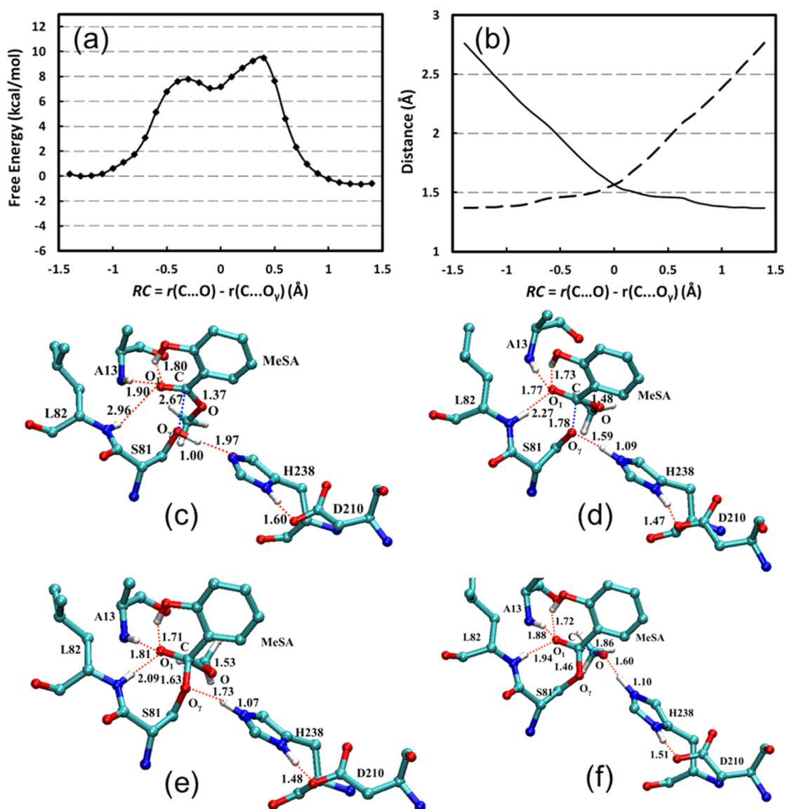
Figure 4. PMF results for SABP2 complexed with MeSA with SCC-DFTB/MM. (a) The free energy profile along the reaction coordinate. See Figure S1A for the same profile with error bars. (b) Changes in the average distances along the reaction coordinate: (—) r(\text{C}\cdots\text{O}_\gamma) and (---) r(\text{C}\cdots\text{O}) . (c) Average structure of the reactant state. (d) Average structure near the first transition state. (e) Average structure of the tetrahedral intermediate. (f) Average structure near the second transition state. Most hydrogen atoms have been omitted for the sake of clarity. Distances are in angstroms, and free energies are in kilocalories per mole.
